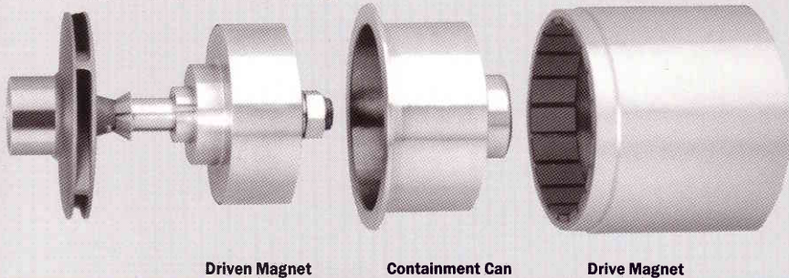
Driven Magnet
